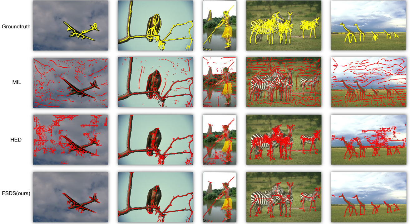
Figure 8. Illustration of skeleton extraction results on the SYMMAX300 dataset [31] for several selected images. The groundtruth skeletons are in yellow and the thresholded extraction results are in red. Thresholds were optimized over the whole dataset.
