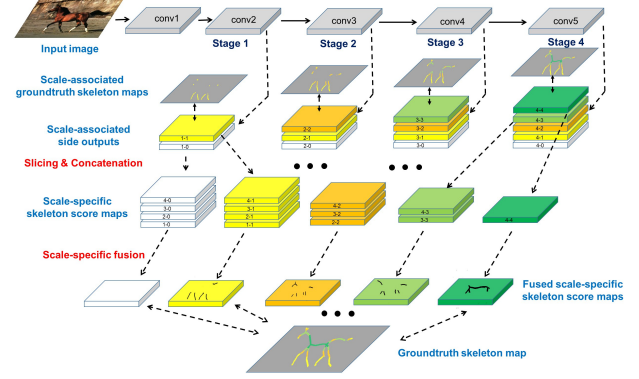
Figure 4. The proposed network architecture for skeleton extraction, which is converted from VGG 16-layer net [28]. It has 4 stages with additional scale-associated side output layers connected to the convolutional layers. Each scale-associated side output is guided by a scale-associated groundtruth skeleton map (The skeleton pixels with different quantized scales are in different colors.). Each scale-associated side output layer provides a certain number of scale-specific skeleton score maps (identified by stage number-quantized scale value pairs). The score maps of the same scales from different stages will be sliced and concatenated. Five scale-specific weighted-fusion layers are added to automatically fuse outputs from multiple stages.
