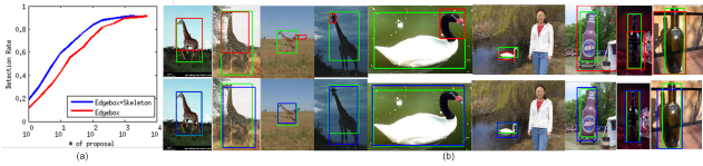
Figure 13. Object proposal results on ETHZ Shape Classes [12]. (a) The curve (IoU = 0.7). (b) Examples. Groundtruth (green), the closest proposal to groundtruth of Edgebox (red) and ours (blue).
