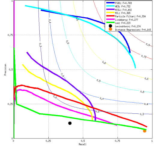
Figure 9. Evaluation of skeleton extractors on the WH-SYMMAX Dataset [25]. Leading skeleton extraction methods are ranked according to their best F-measure with respect to groundtruth skeletons. Our method, FSDS achieves the top result and shows both improved recall and precision at most of the precision-recall regime. See Table 2 for more details about the other two quantities and method citations.
