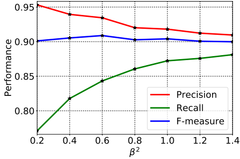
Figure 6. Precision , Recall , F-measure of model trained under different \beta^2 (Eq. 1). The precision decreases with the growing of \beta^2 whereas recall increases. This characteristic gives us much flexibility to adjust the balance between recall and precision: use larger \beta^2 in a recall-first application and lower \beta^2 otherwise.
