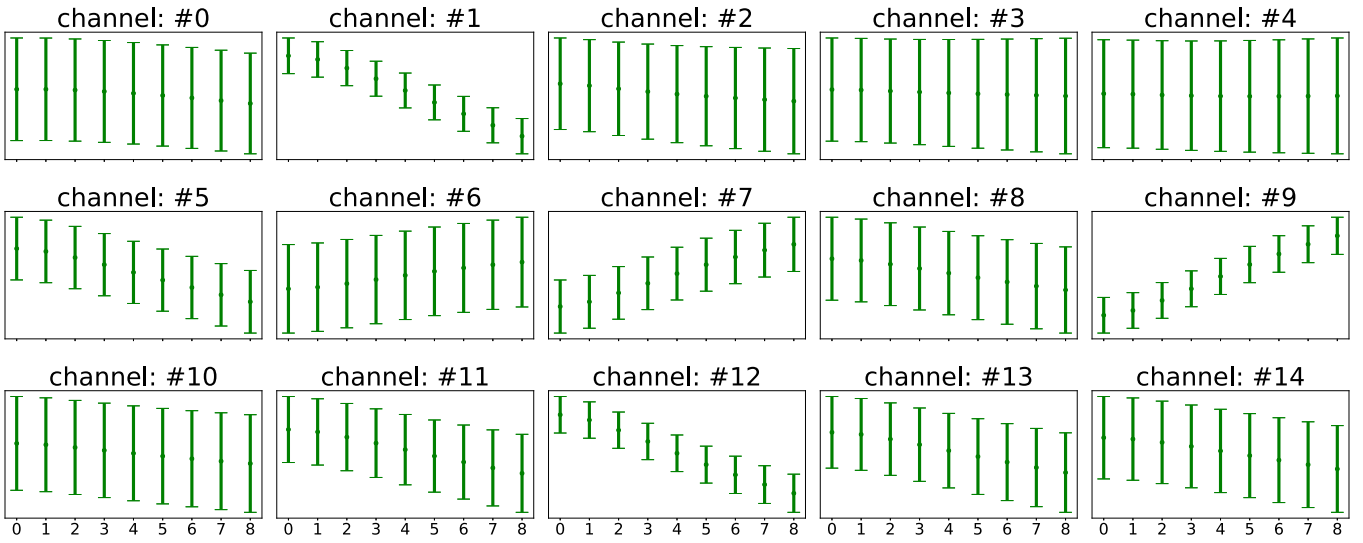
Fig. 3. Per-channel mean and variance of intermediate convolution features under different attacking strengths. Features under different attacking strengths undergo a continuous domain transfer.
