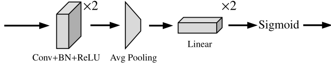
Fig. 5. Architecture of the weight generator (WG). The cube represents the ‘Convolution → batchnorm → ReLU’ sequential, the trapezoid represents the ‘global average pooling’ and the bar represents the ‘Linear → ReLU’ combo. The output is normalized by the sigmoid function.
