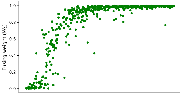
Fig. 6. Relationship between fusion weight W_i and attacking strength \epsilon . With the rising of \epsilon , W_i increases, the features are biased towards the adversarial BN branch, e.g. \text{BN}_{k-1} .
