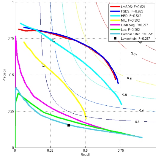
Fig. 10. Skeleton localization evaluation of skeleton extractors on SK-SMALL, which consists of 300 training and 206 testing images. Skeleton extraction methods are measured by their best F-measure with respect to groundtruth skeletons. FSDS and LMSDS achieve the top and the second best results, respectively. See Table III for more details about the other quantity (Avg Runtime) and citations to competitors.
