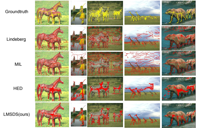
Fig. 11. Illustration of skeleton extraction results on the SYMMAX300 dataset [15] for several selected images. The groundtruth skeletons are in yellow and the thresholded extraction results are in red. Thresholds were optimized over the whole dataset.
